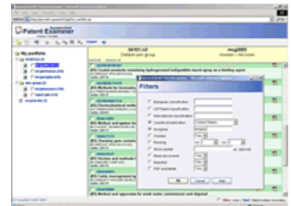
Filtering feature
