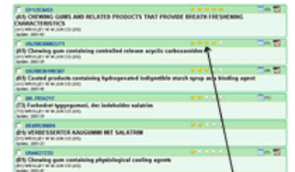
Sorted Ranking
